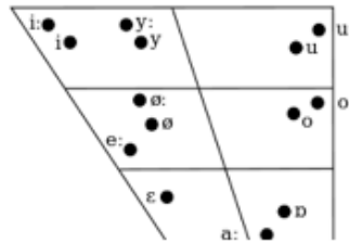
Hungarian Vowels
